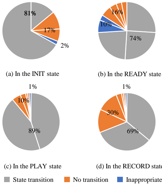
Fig. 5. The next types of client requests generated by the LLM in each state. The types in gray induce state transitions, the ones in orange appear in the suitable state but do not trigger state transitions, and the ones in blue appear in the inappropriate states. Each segment represents one distinct message type.
